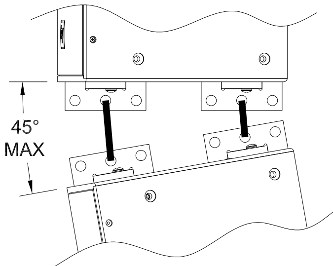
Figure 34: Box-to-Box internal connection points of a horizontal cluster using HRK horizontal rigging kits
